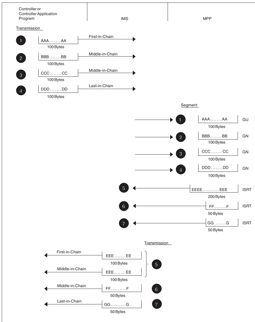
Figure 64. Chained Message Interaction between a Finance Communication System and an IMS MPP
